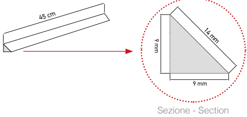
Dettaglio quarter round - Quarter round detail
